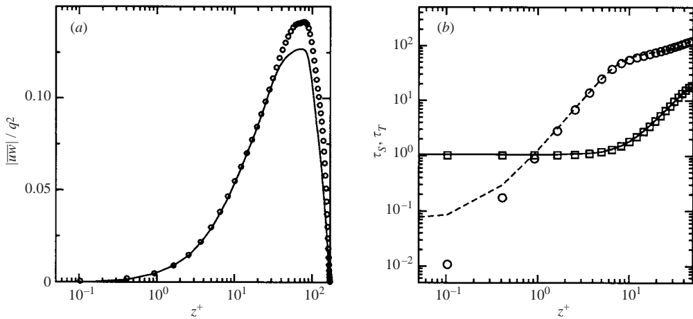
FIGURE 23. (a) Profiles of the structure parameter |\overline{u'w'}|/q^2 . Lines and symbols are used to identify FDI and OCH, respectively. (b) Time scales. — and \square , \tau_S ; --- and \circ , \tau_T .
