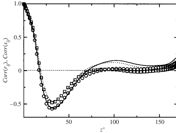
FIGURE 11. Profiles of the autocorrelation function between the \langle r_{ij}r_{ij} \rangle and \langle s_{ij}s_{ij} \rangle at the interface/wall and that in the bulk flow. Lines and symbols are used to identify FDI and OCH, respectively. — and \circ , Corr(r_{ij}) ; \cdots and \square , Corr(s_{ij}) .
