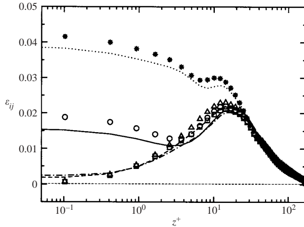
FIGURE 8. Profiles of the off-diagonal components of the dissipation tensor. Lines and symbols are used to identify FDI and OCH, respectively. — and \circ , \epsilon_{12} ; --- and \square , \epsilon_{13} ; ··· and \triangle , \epsilon_{23} ; ··· and * , \epsilon .
