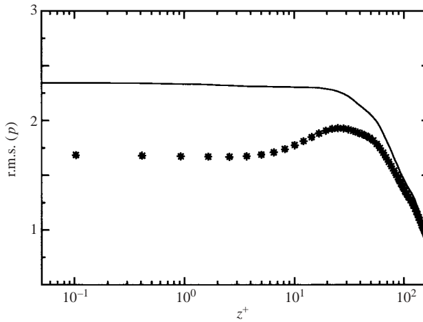
FIGURE 12. Profiles of the r.m.s. pressure fluctuation, p . Lines and symbols are used to identify FDI and OCH, respectively.
