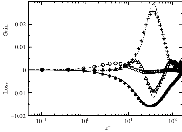
FIGURE 17. Terms in the budget for \overline{w\overline{w}} in wall units. Lines and symbols are used to identify FDI and OCH, respectively. — and *, dissipation; -·-·- and +, pressure diffusion; ---- and \Delta , turbulent diffusion; - - - and \circ , viscous diffusion.
