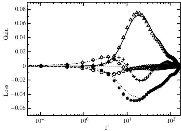
FIGURE 18. Terms in the budget for \overline{u\overline{w}} in wall units. Lines and symbols are used to identify FDI and OCH, respectively. — and \Delta , production; ---- and \circ , dissipation; - - - and \diamond , viscous diffusion; ··· and *, pressure diffusion; -·-·- and +, turbulent diffusion.
